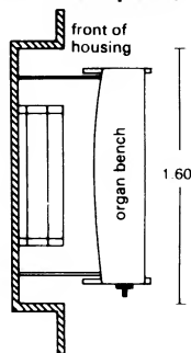
10 Plan of manual console
